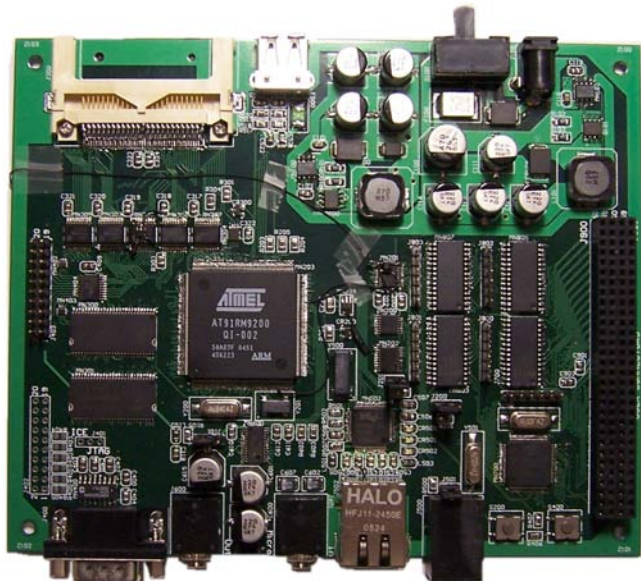
Figure 4: ARMUS' hardware.
